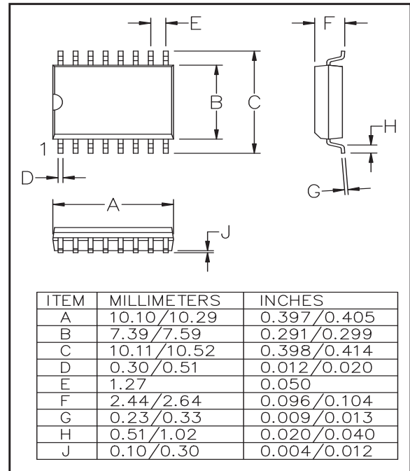
Figure 6. 16-pin SO Wide package outline
