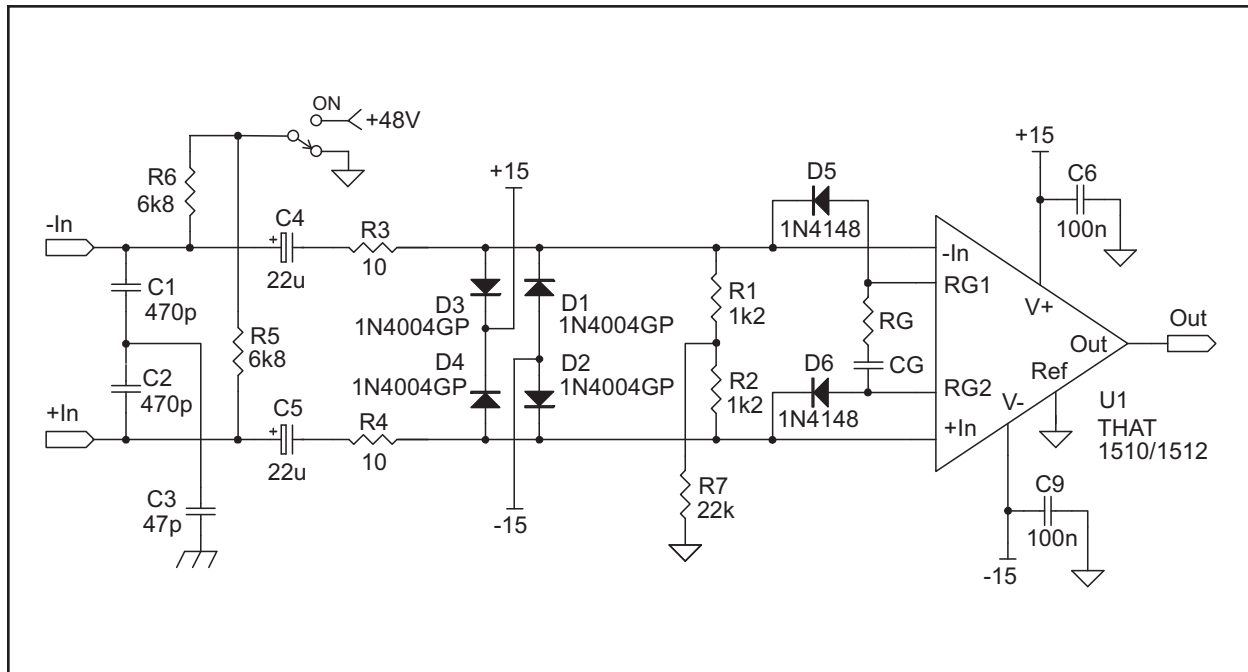
Figure 4. Recommended 1510 / 1512 Circuit with Phantom Power
